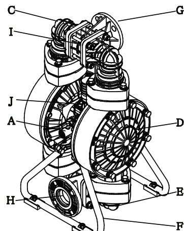
NDP-H50BP□
