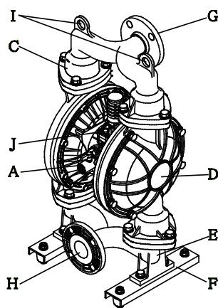
NDP-H40BS□
