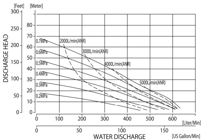
■ NDP-50BAW/BSW/BFW
