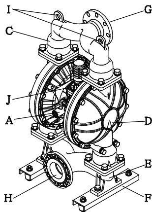
NDP-H80BS□
