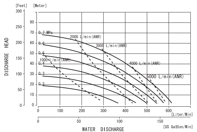
■ NDP-50BP□/BV□
