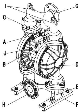
NDP-40BS□ NDP-40BF□
