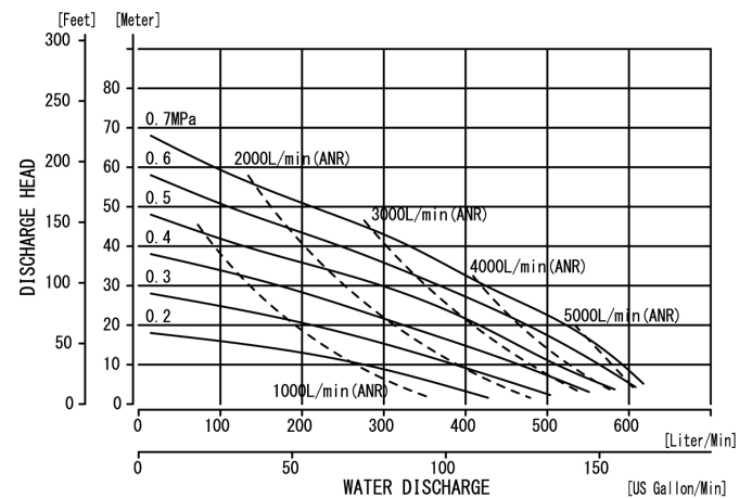
■ NDP-50BPW/BVW
