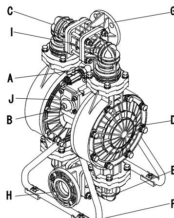
NDP-40BP□ NDP-40BV□
