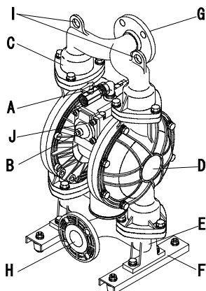
NDP-50BS□ NDP-50BF□
