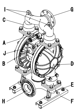
NDP-80BS□ NDP-80BF□
