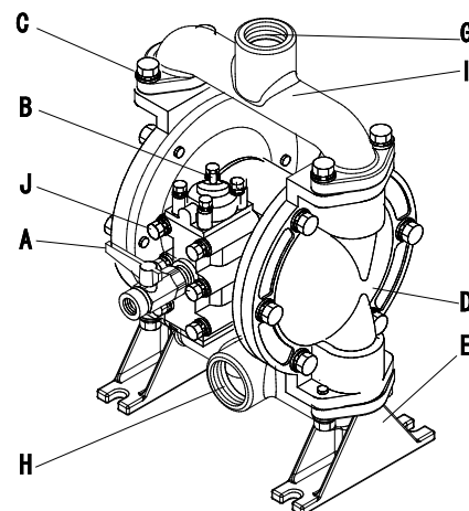
NDP-32BAN NDP-32BAT
