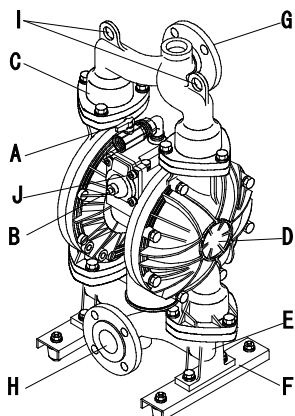
NDP-50BA□
