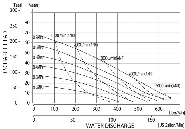
■ NDP-50BA□/BS□/BF□
