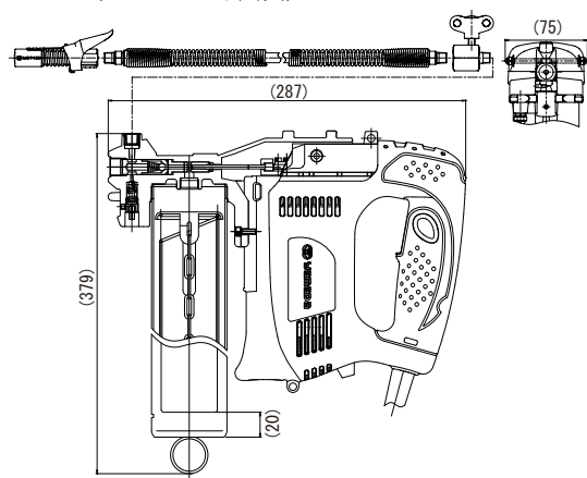
(EG-400A II 寸法図)
