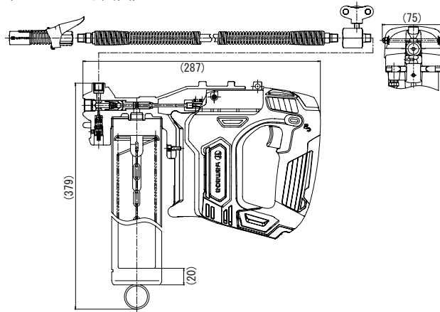
(EG-400B II 寸法図)
