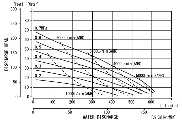
■ NDP-50BPW/BVW
