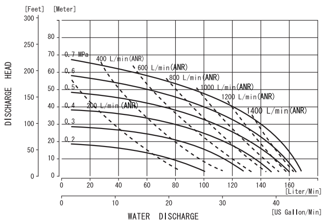
■ NDP-25BA□/BS□/BF□/BP□/BV□
