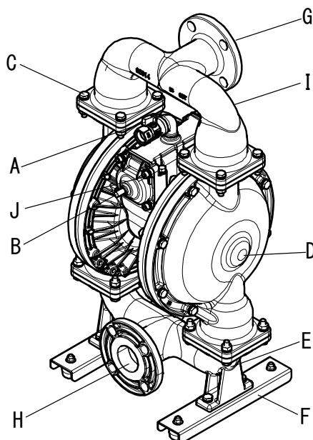
NDP-500BS□
