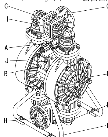
NDP-40BP□ NDP-40BV□
