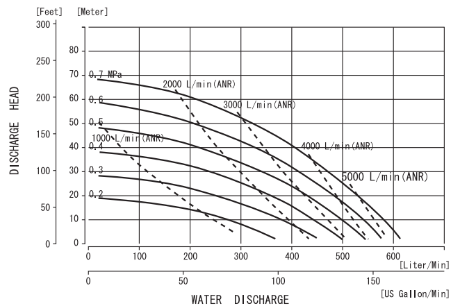
■ NDP-50BP□/BV□
